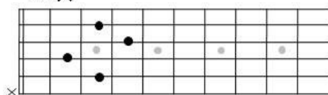
CM7[9]
