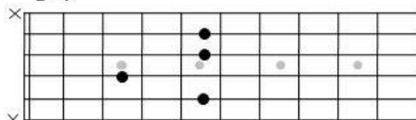
Dm9
