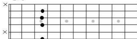
Gm7
