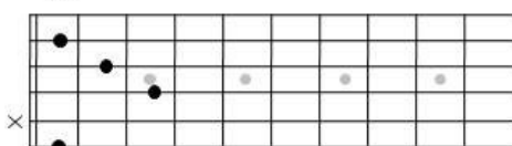
FM7
