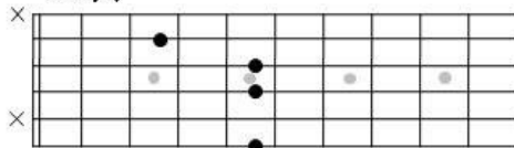
Am7[11]
