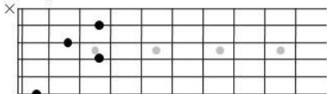
Fm6
